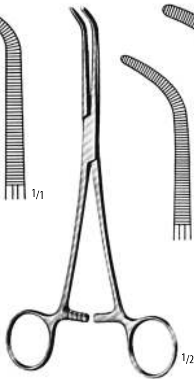
MIXTER - O'SHAUGHNESSY 15,5 cm / 6" HM - 521 - 15 19,0 cm / 7 1/2" HM - 521 - 19
