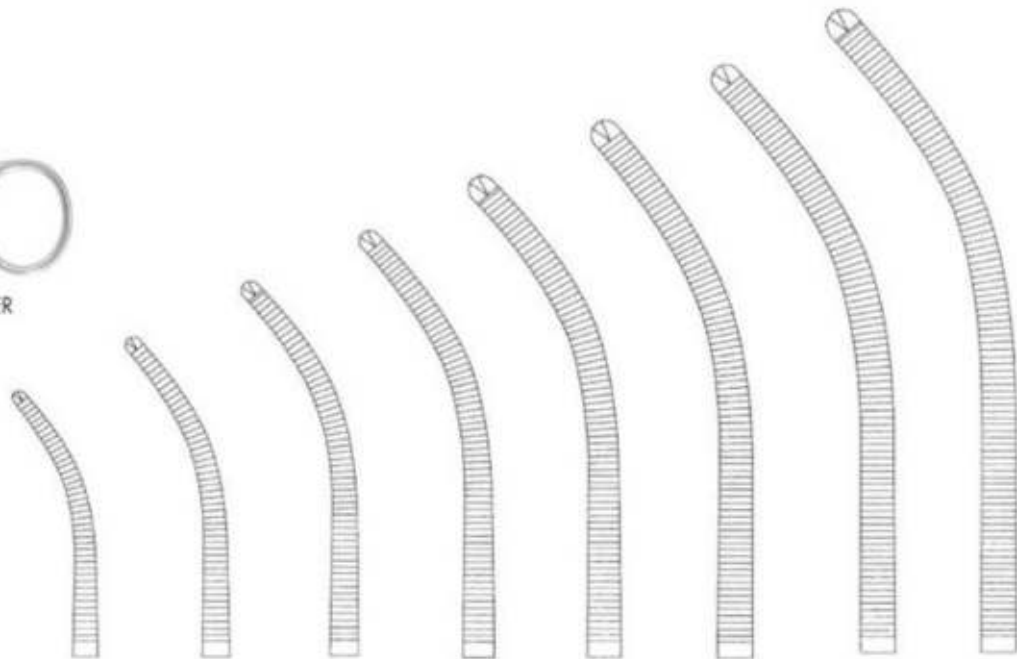
HM 406-14 HM 406-16 HM 406-18 HM 406-20 HM 406-22 HM 406-24 HM 406-26 HM 406-30 14 cm/5½" 16 cm/6¼" 18 cm/7" 20 cm/8" 22 cm/8¾" 24 cm/9½" 26 cm/10¼" 30 cm/12"
